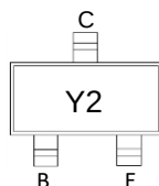
Marking and pin assignment
